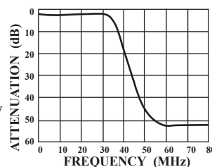
MFJ-705 Frequency Response
