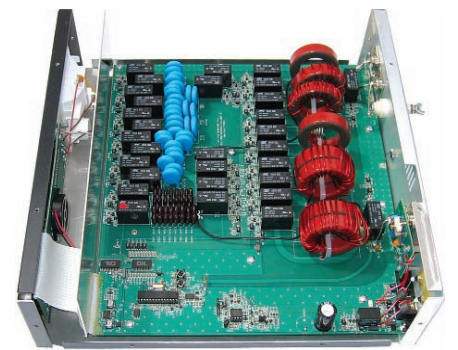
An Inside view of MFJ-998
