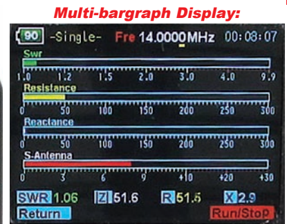
SWR, R, X and Z are simultaneously displayed in vivid color graphs.
